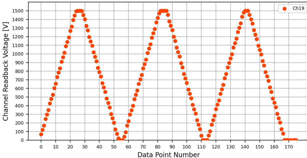
Voltage Ramp Test (Python) Bd #081, Slot #4, Ch #19
