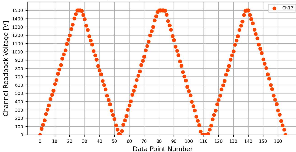
Voltage Ramp Test (Python) Bd #081, Slot #4, Ch #13
