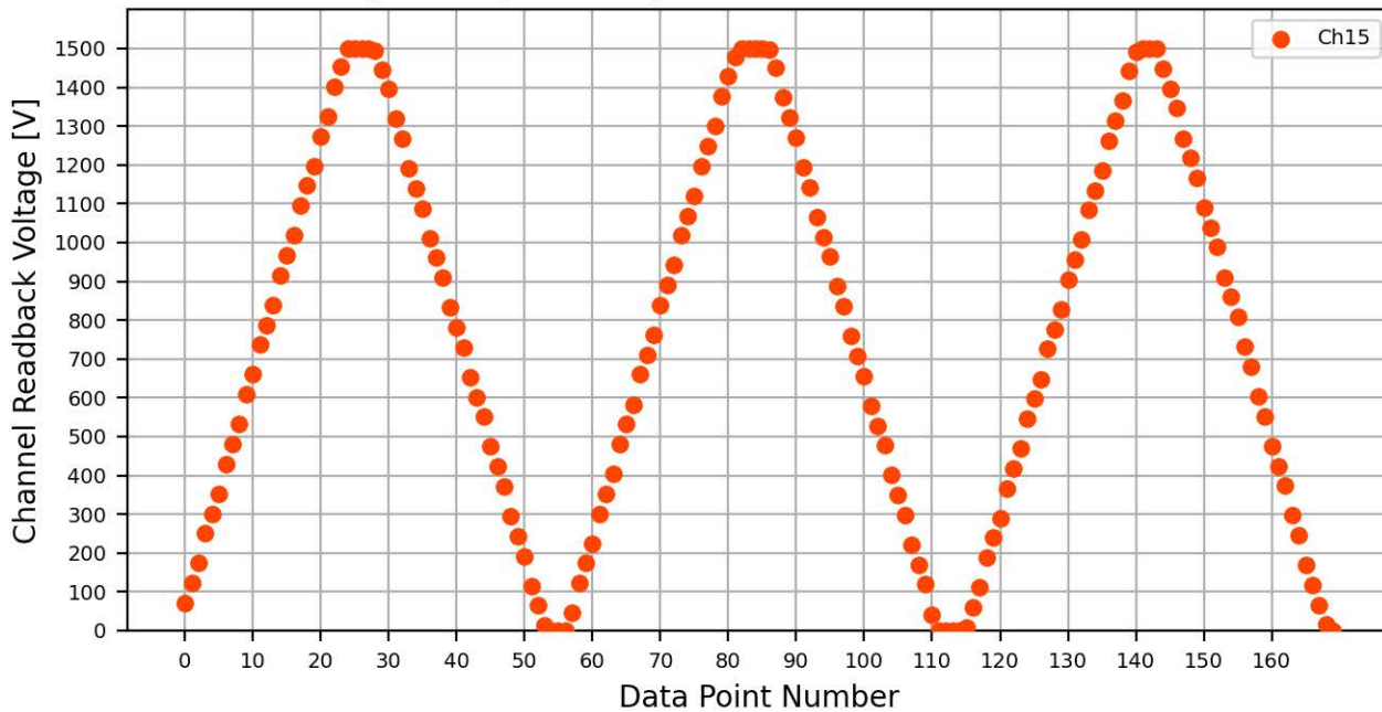
Voltage Ramp Test (Python) Bd #081, Slot #4, Ch #15
