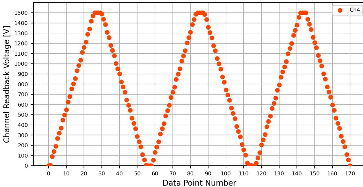
Voltage Ramp Test (Python) Bd #081, Slot #4, Ch #4
