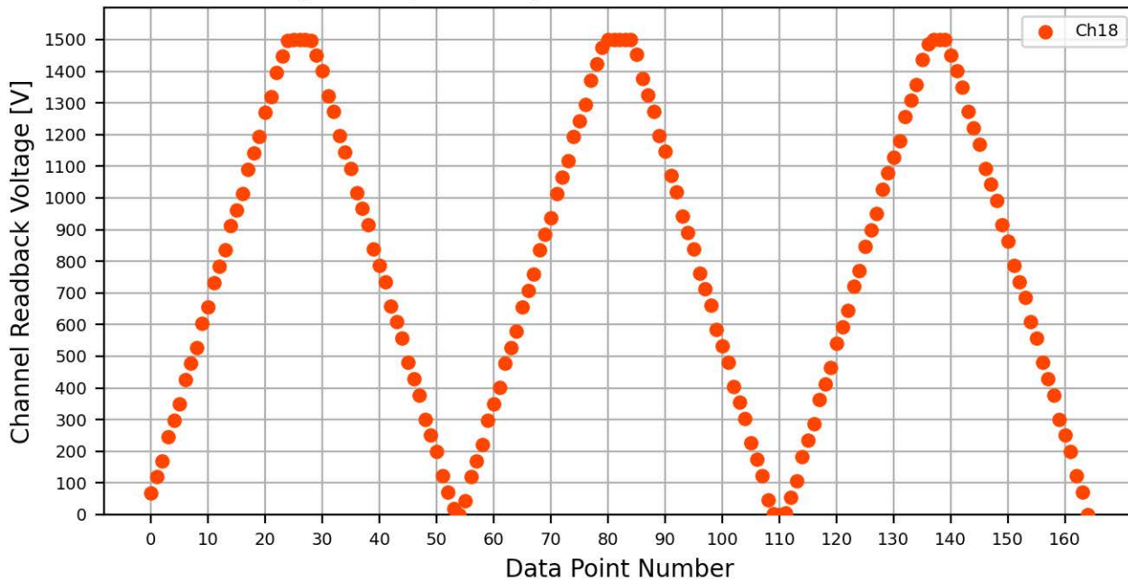
Voltage Ramp Test (Python) Bd #081, Slot #4, Ch #18
