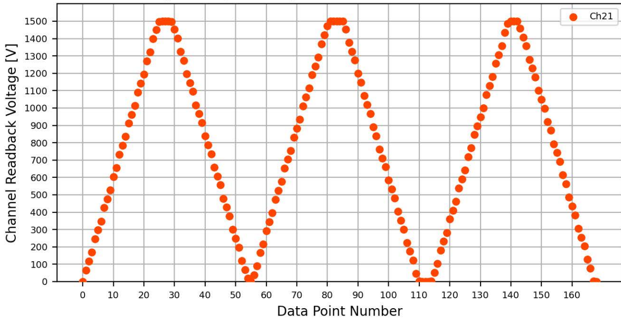
Voltage Ramp Test (Python) Bd #081, Slot #4, Ch #21
