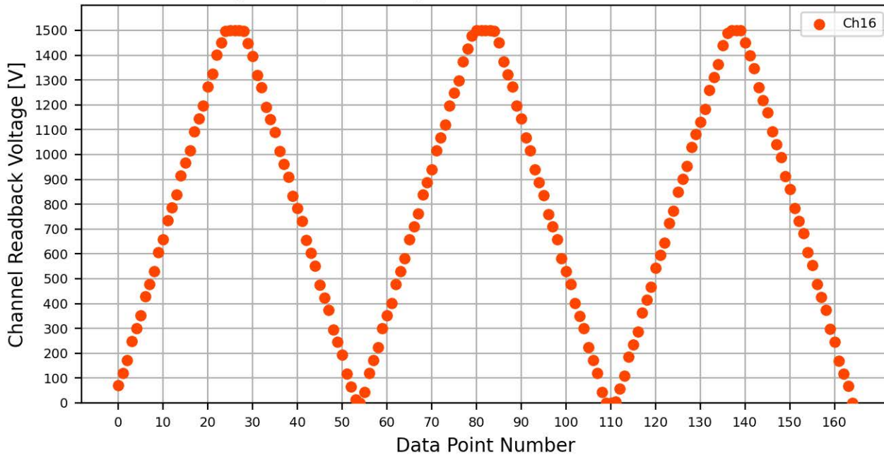
Voltage Ramp Test (Python) Bd #081, Slot #4, Ch #16
