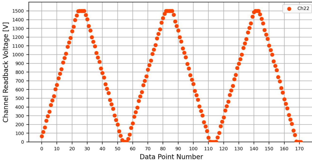
Voltage Ramp Test (Python) Bd #081, Slot #4, Ch #22
