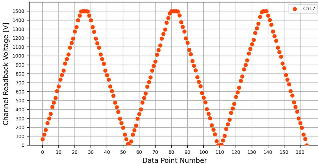
Voltage Ramp Test (Python) Bd #081, Slot #4, Ch #17
