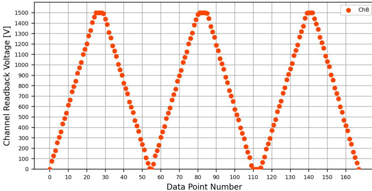
Voltage Ramp Test (Python) Bd #081, Slot #4, Ch #8
