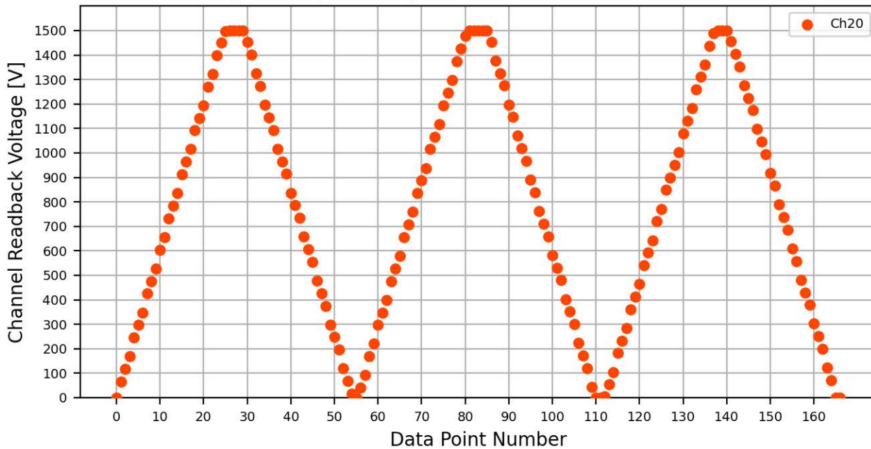
Voltage Ramp Test (Python) Bd #081, Slot #4, Ch #20
