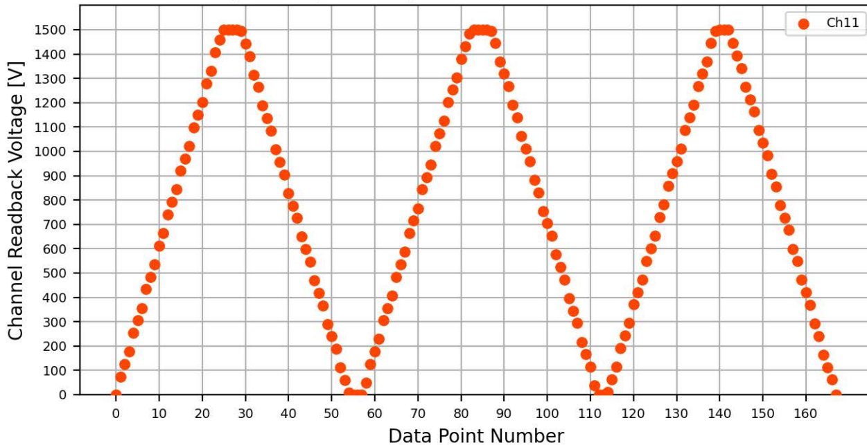
Voltage Ramp Test (Python) Bd #081, Slot #4, Ch #11
