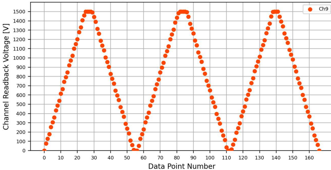
Voltage Ramp Test (Python) Bd #081, Slot #4, Ch #9
