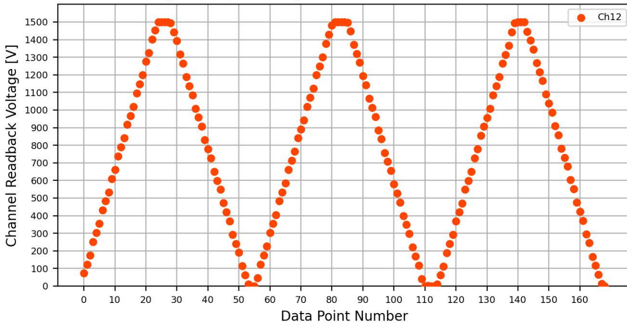
Voltage Ramp Test (Python) Bd #081, Slot #4, Ch #12
