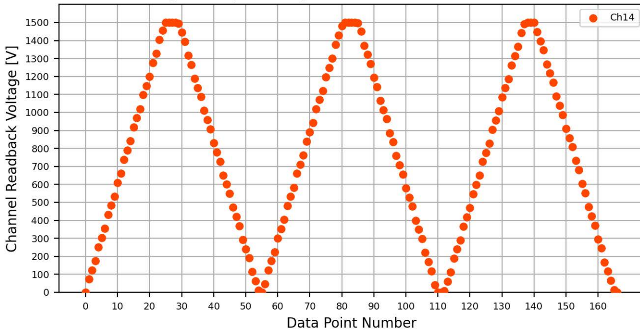
Voltage Ramp Test (Python) Bd #081, Slot #4, Ch #14
