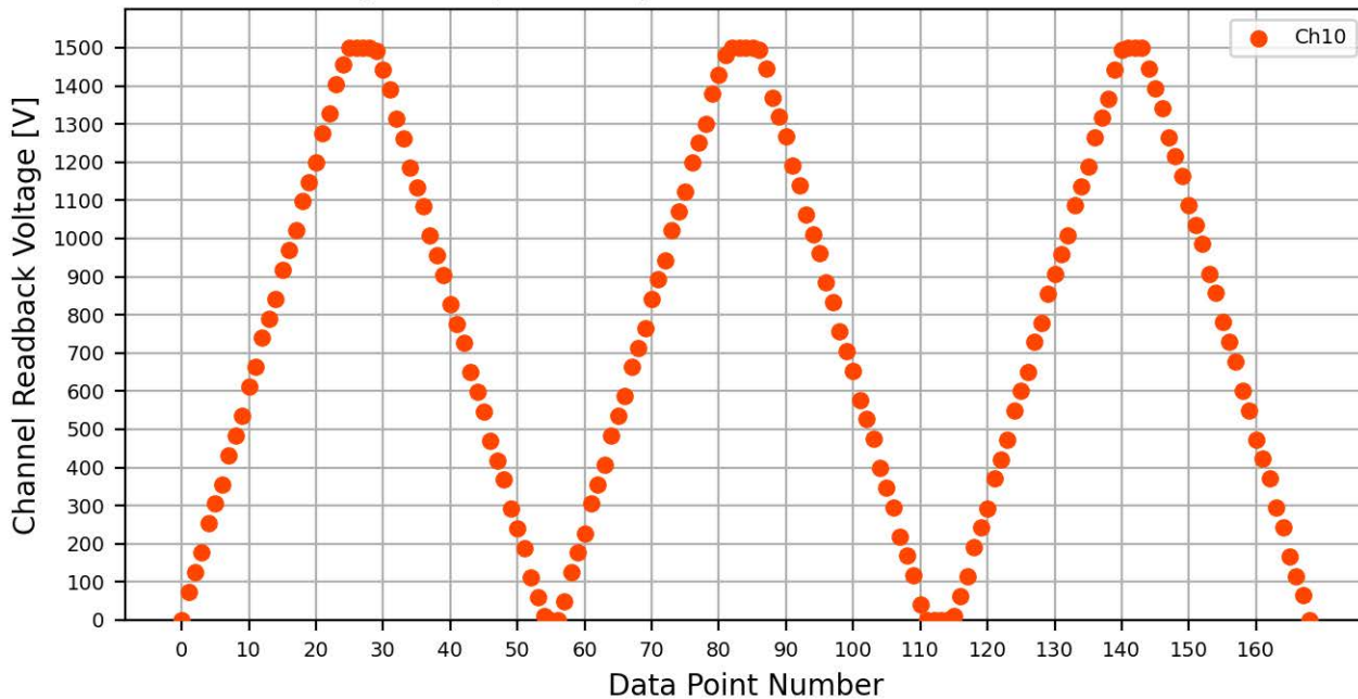
Voltage Ramp Test (Python) Bd #081, Slot #4, Ch #10
