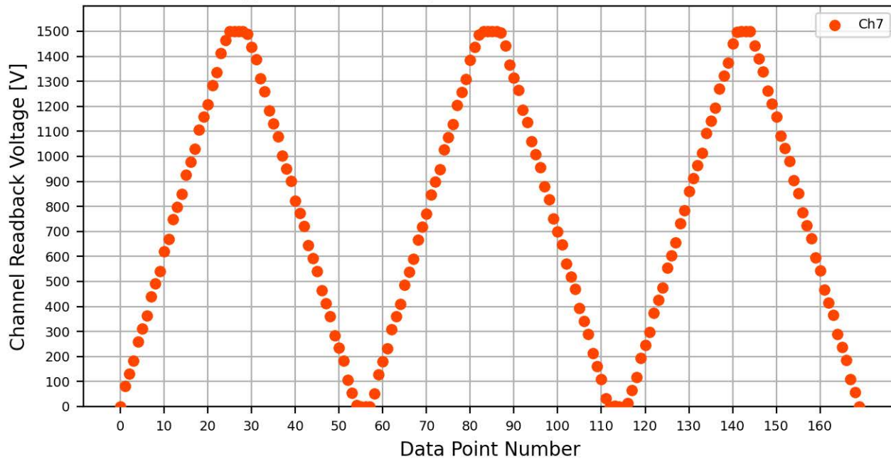
Voltage Ramp Test (Python) Bd #081, Slot #4, Ch #7
